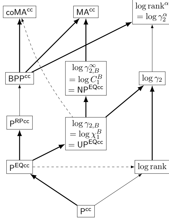
Figure 2: Relationships between the communication complexity measures. We consider total functions only. \mathcal{A} \rightarrow \mathcal{B} with a normal arrow represents \mathcal{A} \subseteq \mathcal{B} . The arrow is bold if that inclusion is known to be strict ( \mathcal{A} \subsetneq \mathcal{B} ). The arrow is dashed if a separation is known ( \mathcal{A} \not\subseteq \mathcal{B} ). Some relationships are omitted if they can be derived from the others shown here.
